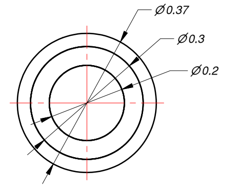
VIEW A FIBER CONSTRUCTION EXAMPLE: ZLPUV200/300N//370
